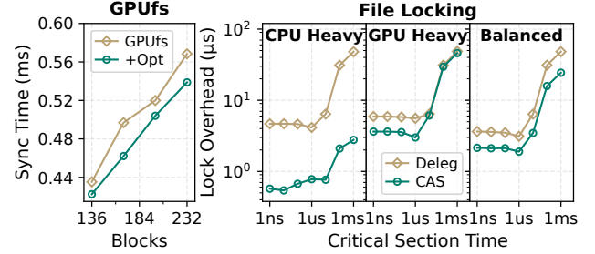
Figure 13. Control-plane optimization for GPUfs and file locking on Orin. Deleg denotes Delegation on the right figure.
