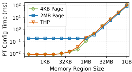
Figure 1. Page table configuration time for the GPU using different page sizes on Spark.
