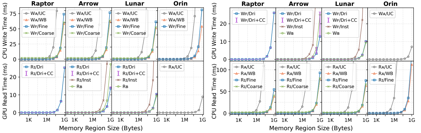
Figure 6. Performance of WRITE and READ implementations for memory sharing from CPU to GPU (left) and from GPU to CPU (right). Vertical bars mark the GPU time overhead from enabling CC on Raptor, Arrow, and Lunar.
