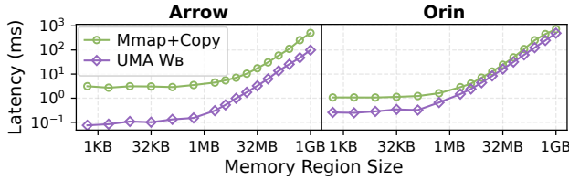
Figure 7. Performance of CPU WRITE from SSD to memory.
