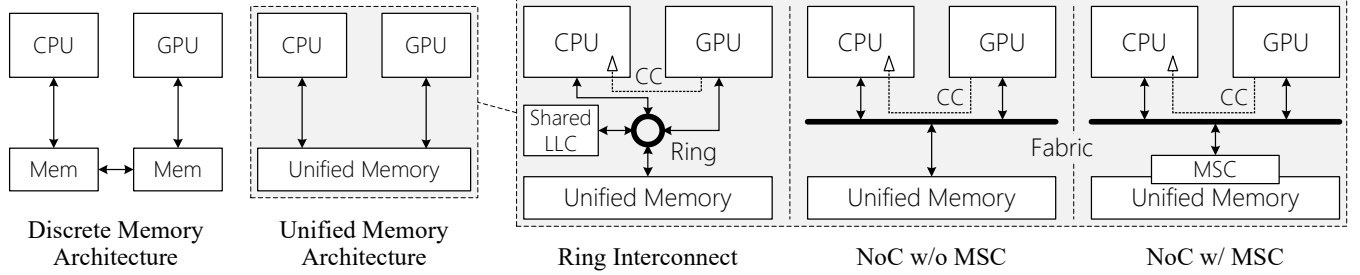
Figure 2. Discrete memory architecture, unified memory architecture (UMA), and UMA with different hardware features. All interconnect panels are logical views; e.g., the shared LLC on the ring is physically sliced across ring stops co-located with cores.
