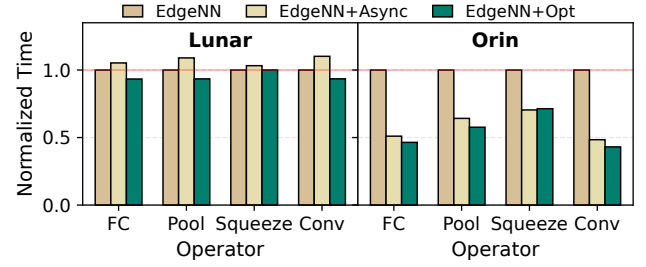
Figure 11. Control-plane optimization for hybrid inference on Lunar (left) and Orin (right).
