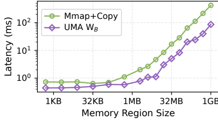
Figure 3. Performance of CPU WRITE from SSD to memory on Spark. W_B reduces end-to-end loading time relative to the mmap-and-copy path by avoiding extra staging and copy overhead.
