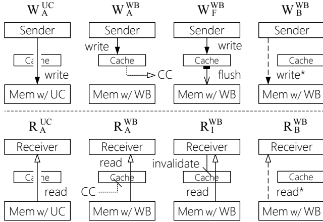
Figure 4. Different implementations of WRITE and READ.
