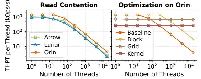
Figure 8. GPU R_B performance as the thread count increases. The number of threads per block is up to 256.
