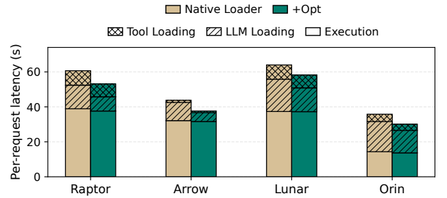
Figure 14. Estimated per-request agent-serving latency on TaskBench traces, including three tool calls.
