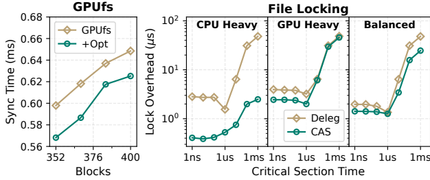
Figure 7. Control-plane coordination for GPUfs and file locking on Spark. Deleg denotes the delegation lock in the right-hand plot.
