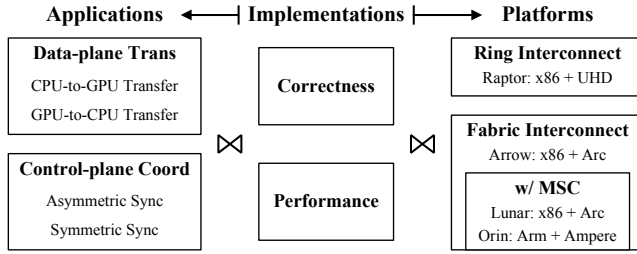
Figure 1. Our analysis methodology.
