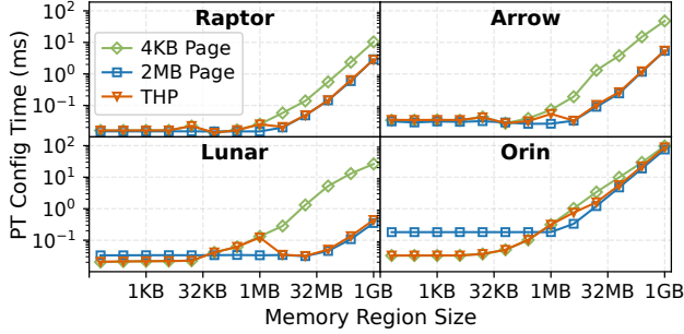
Figure 5. A comparison of page table configuration time for the GPU using different page sizes on our target platforms.
