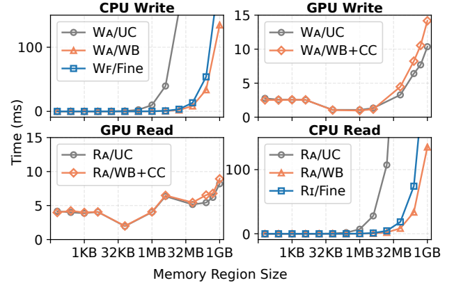
Figure 2. Performance of WRITE and READ implementations for memory sharing on Spark, broken down by CPU and GPU access paths. CC denotes two-way coherence.
